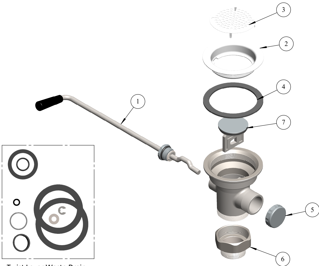
Twist Lever Waste Drain Repair Kit C9501 (Washers, O-Rings & Gaskets are included)
